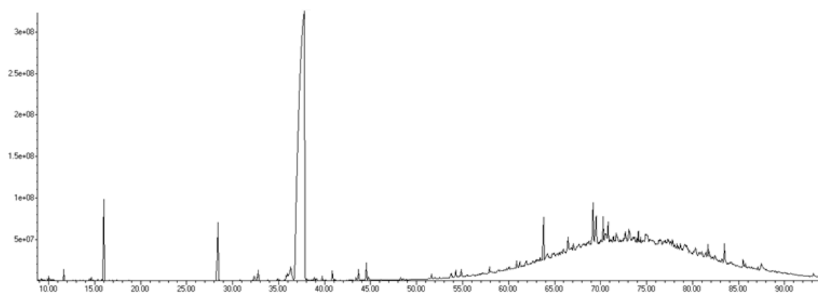
Figure S5. Gas chromatogram of U. dermestoides essential oil under T1 stimuli (EOT1).
