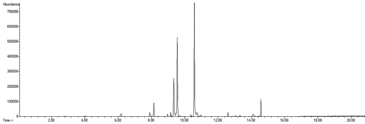
Figure S1. Gas chromatogram of the HS-SPME (CAR/PDMS fiber) at 1h of U. dermestoides under T1 treatment.
