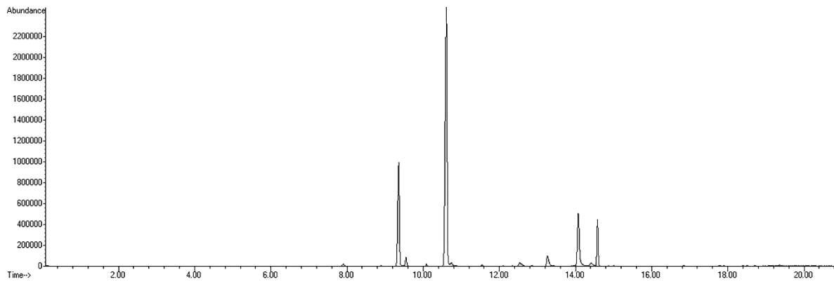
Figure S2. Gas chromatogram of the HS-SPME (PEG fiber) at 1h of U. dermestoides under T1 treatment.
