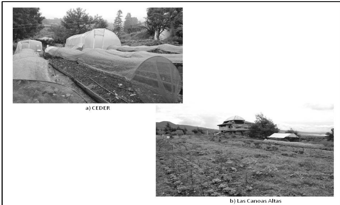
Figure 20: Drip irrigation
